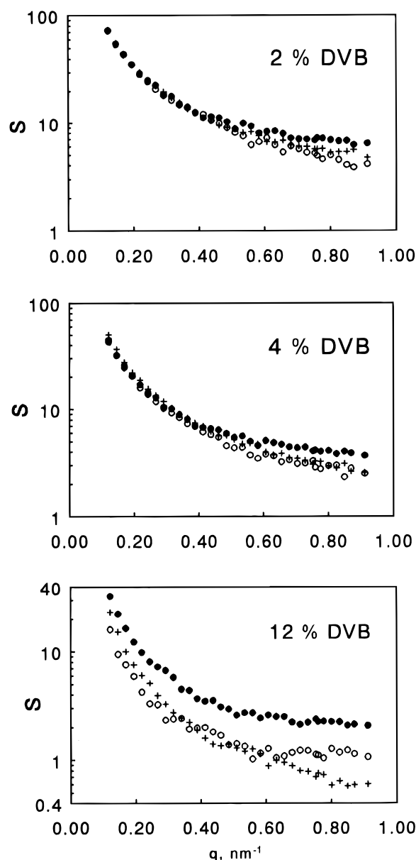
Figure 5. Partial structure functions in the low q range. From top to bottom: 2, 4, and 12% cross-linkages, respectively. The symbols refer to the polymer (●), polymer counterion (+), and counterion (○) partial structure functions.
