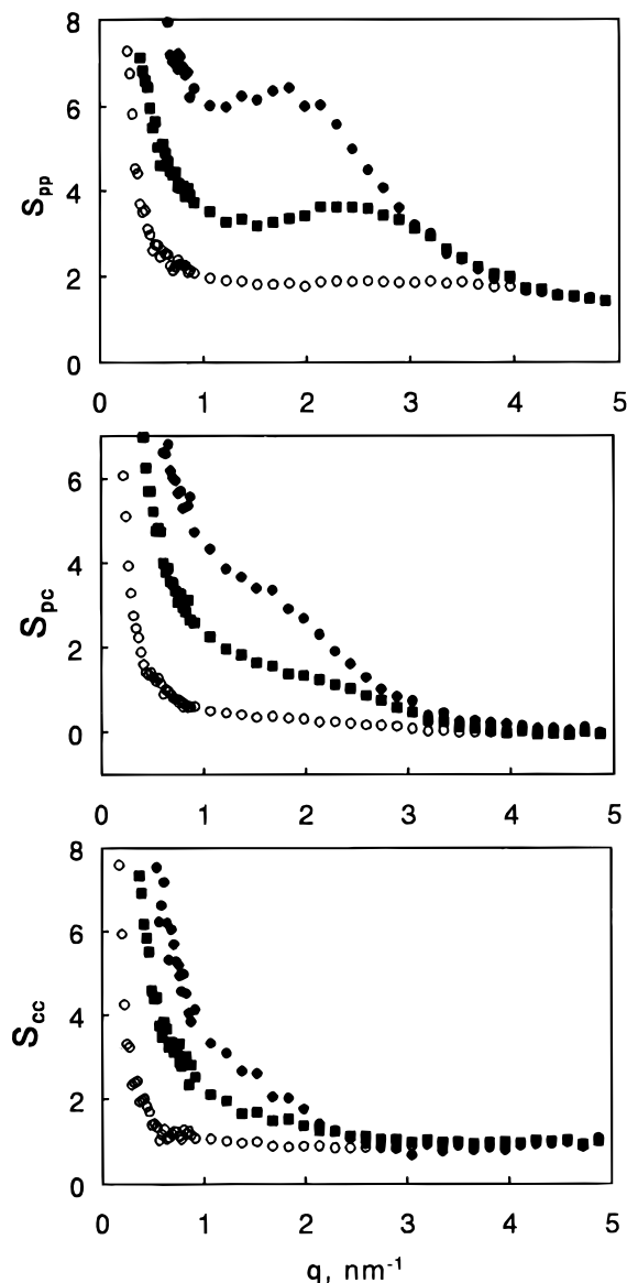
Figure 6. Partial structure functions in the high q range. From top to bottom: polymer, polymer counterion, and counterion partial structure functions. The symbols refer to cross-linkages: \bullet , X-2; \blacksquare , X-4; \circ , X-12.
